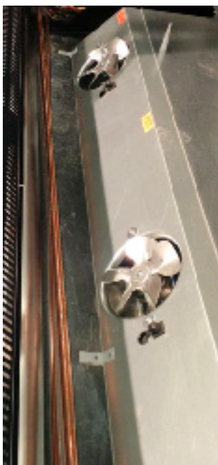
FIGURE 29: Fans and Case-to-Case Piping
