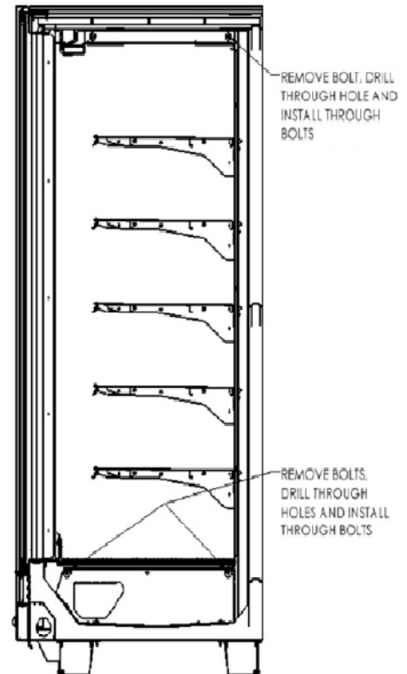
FIGURE 16: Through Bolt Locations
