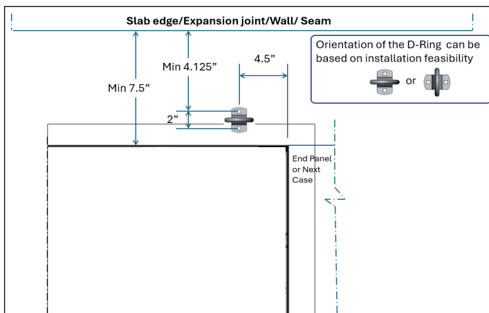
FIGURE 5: Floor Rear D-Ring Installation Kit
