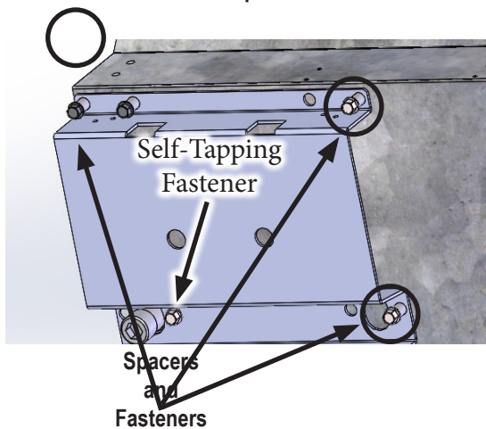
FIGURE 18: Spacer Removal
