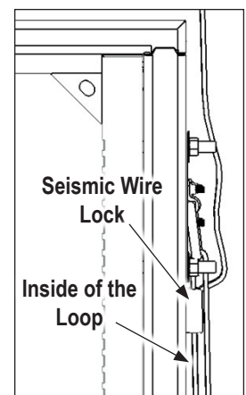
FIGURE 7: D-Ring and Wire Loop View from right-end
