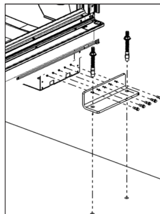
FIGURE 6: Floor Front Seismic Bracket Installation Kit
