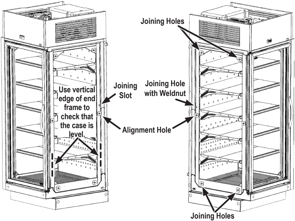
FIGURE 2: 1-Door Guardian Merchandiser
