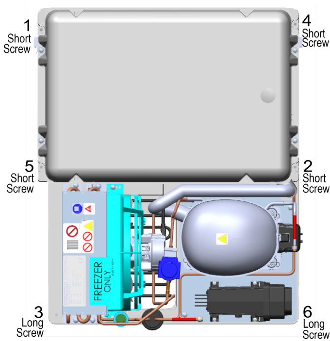
FIGURE 6: 1-Door PRU Mounting Screw Order
