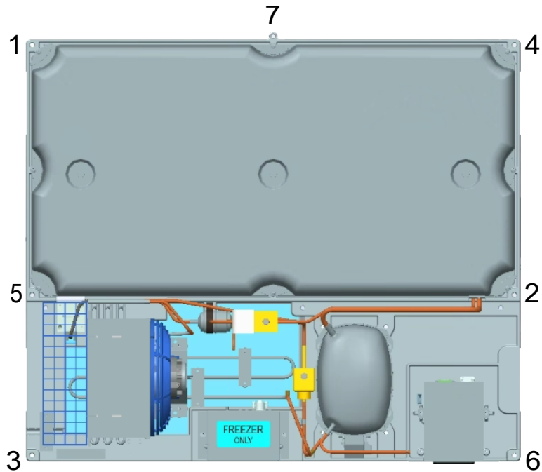
FIGURE 5: Multi-Door PRU Torque Order
