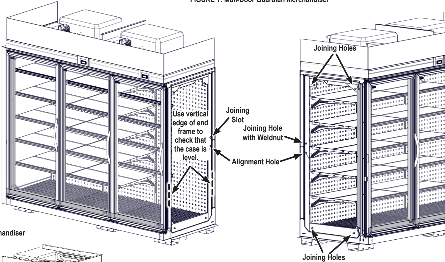
FIGURE 1: Multi-Door Guardian Merchandiser
