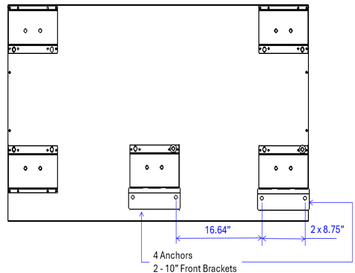
FIGURE 16: 2 Door CGMC30/CGLC30 High Seismic Anchor Layout
