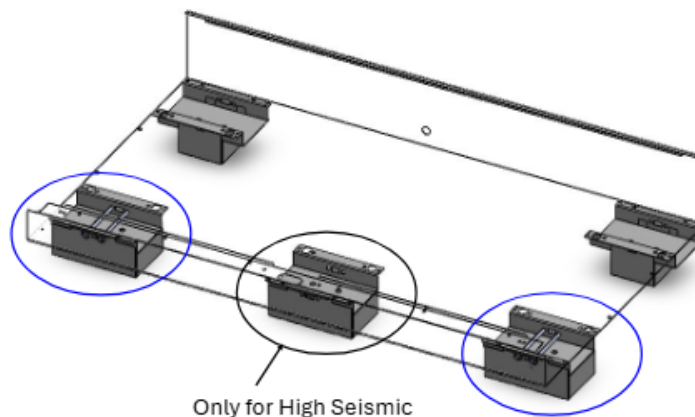
FIGURE 25: Expansion Base Assembly 2-Door View from Front of Case
